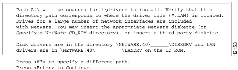
Figure 4-4 Default Driver Path Screen
