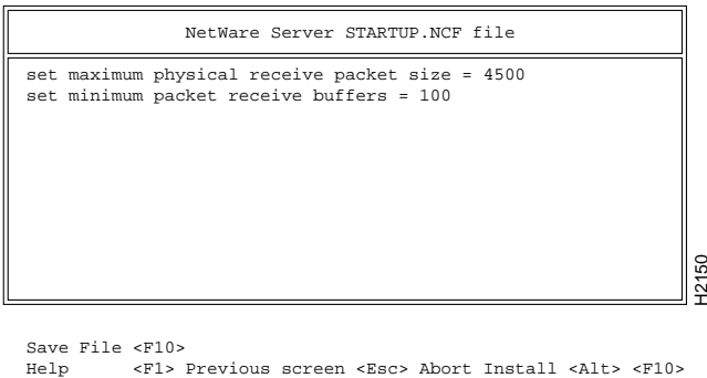
Figure 4-12 NetWare Server STARTUP.NCF File Editing Screen
