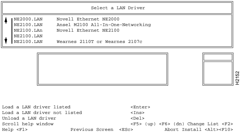
Figure 4-3 Load LAN Driver Entry Screen
