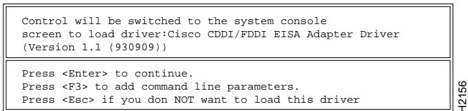
Figure 4-7 Installation Confirmation Screen
