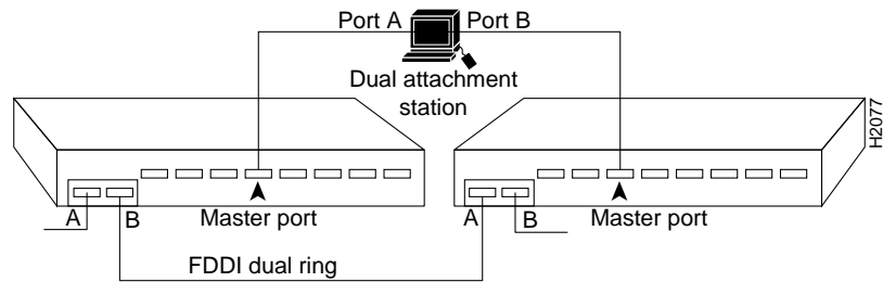
Figure 1-4 Dual Homing
