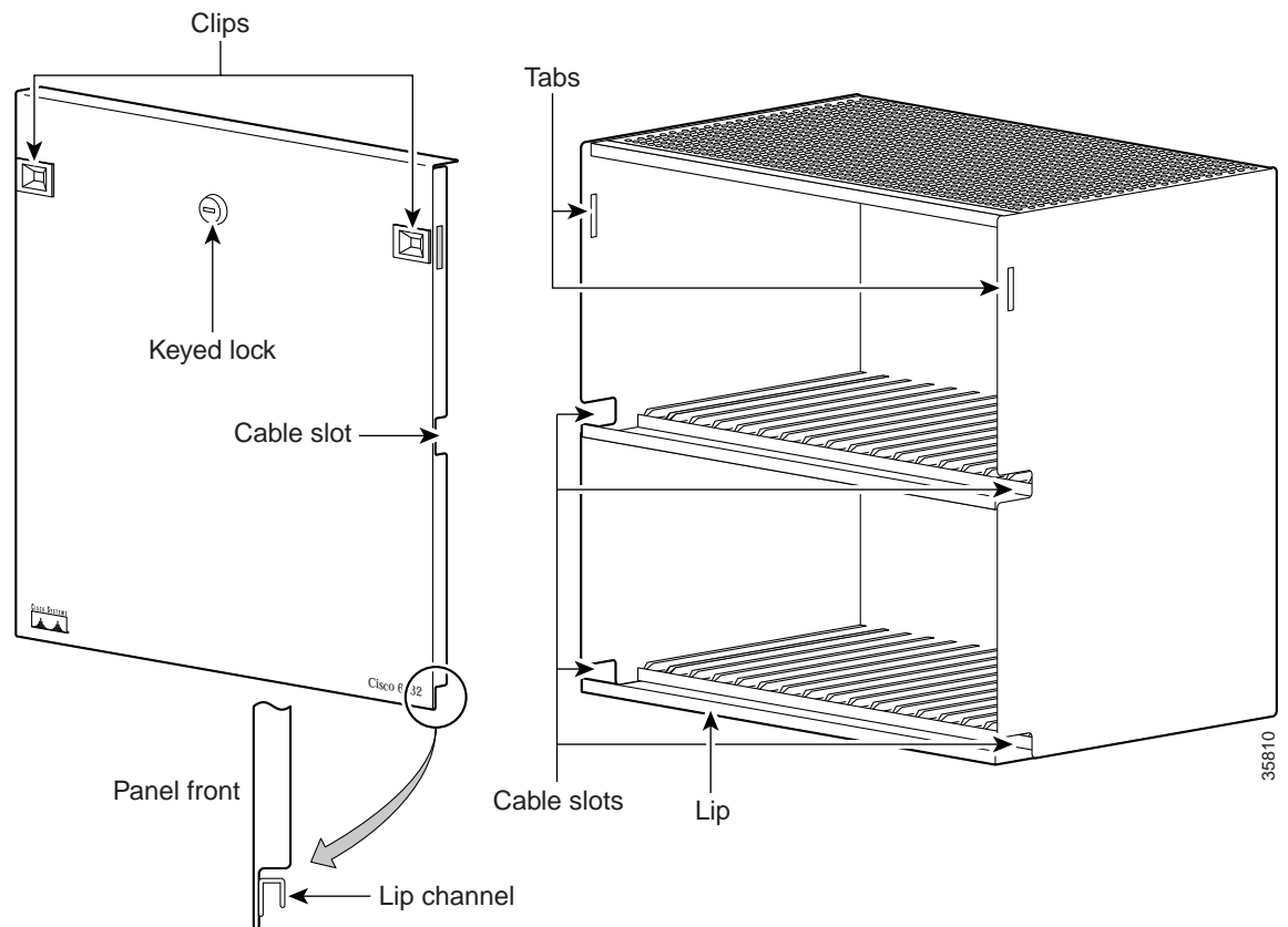
Figure 1 Cisco 6732 Front Panel and Cisco 6732 Chassis
