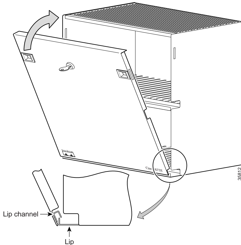
Figure 2 Installing the Front Panel
