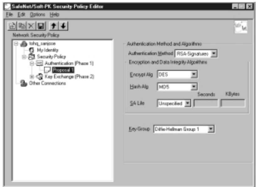
Figure 6-14 Authentication (Phase 1)—Proposal 1 Pane
