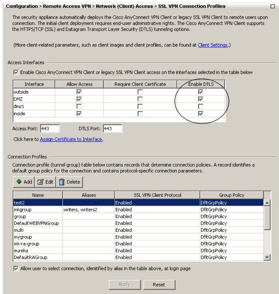
Figure 5-1 Enable DTLS Check Box
