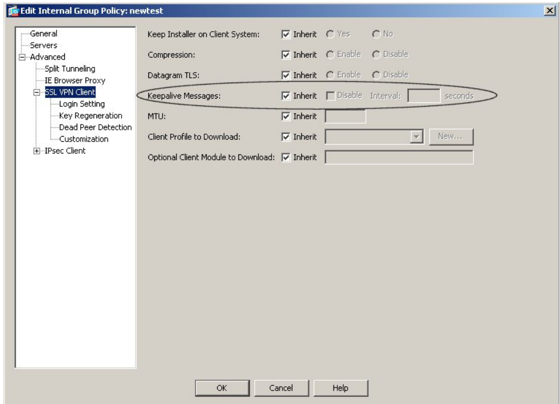
Figure 5-10 Configuring Keepalive Messages
