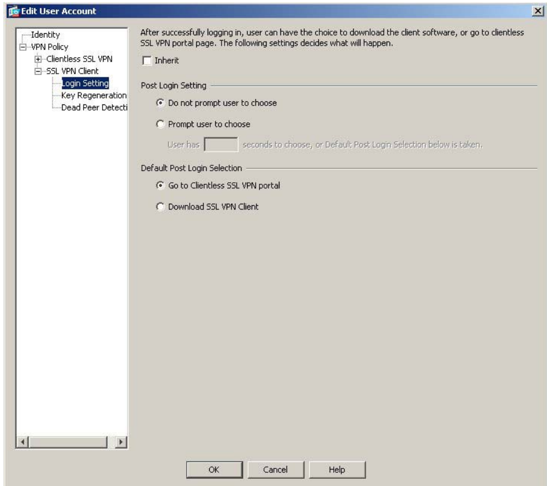
Figure 7-5 Add or Edit User Account Dialog Box (Username)
