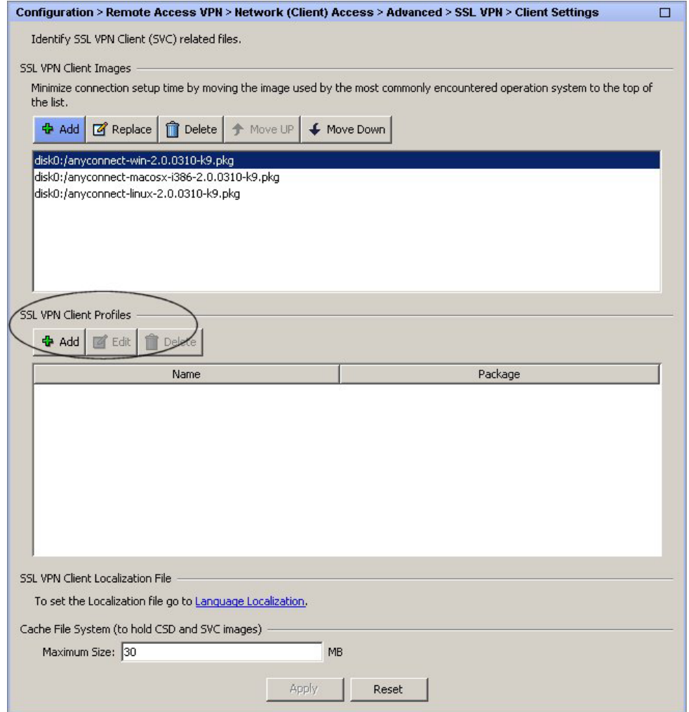
Figure 7-1 Adding or Editing an AnyConnect VPN Client Profile
