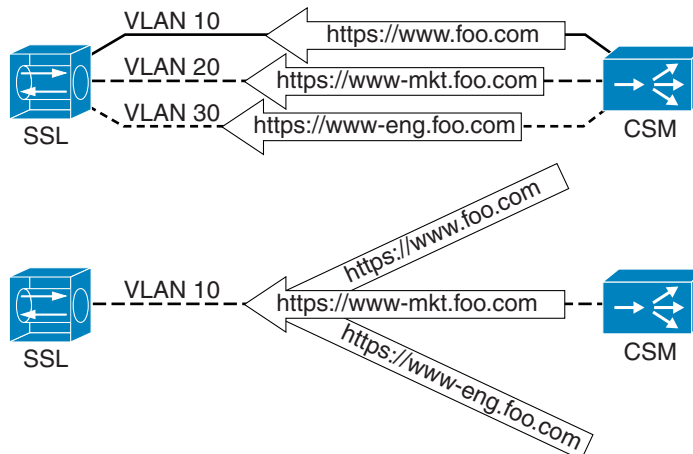
Figure 6-3 Connectivity between the CSM and the SSLSM
