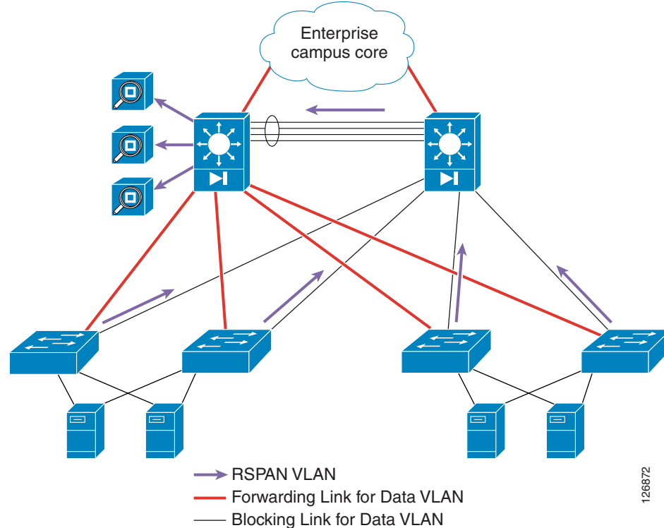
Figure 7-6 RSPAN Design used to Monitor the Locally Switched Traffic on the Access Layer Devices
