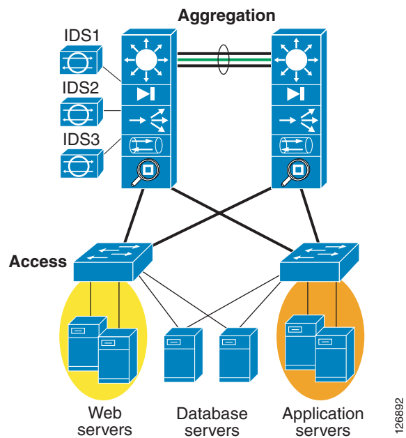
Figure 9-12 Multi-tier Server Farm with Integrated Network Services—Physical Diagram
