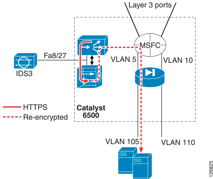
Figure 1-14 Network-based SSL Offloading Combined with IDS Monitoring for HTTPS Inspection
