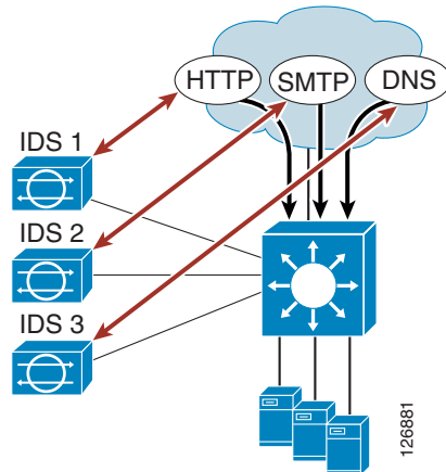
Figure 9-1 Each Sensor Analyzes a Different Protocol
