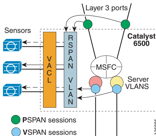
Figure 9-5 Catalyst 6500 Internal Topology with PSPAN Session and VSPAN Session (Not Possible because of CSCdy22529)
