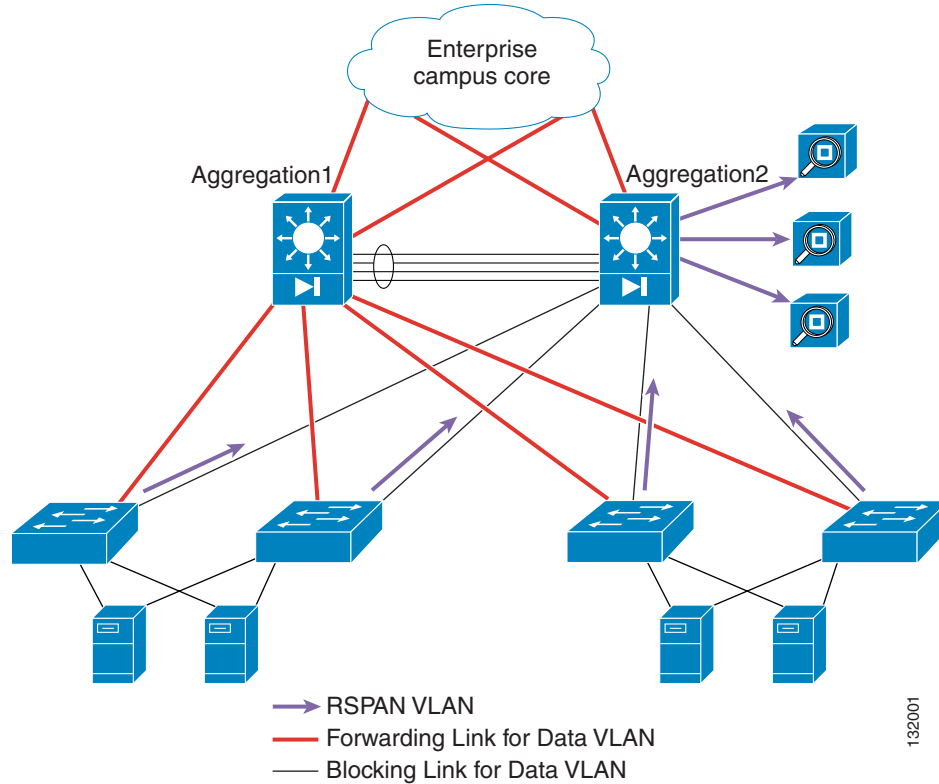
Figure 2-10 Using RSPAN to Monitor Access Switches Traffic
