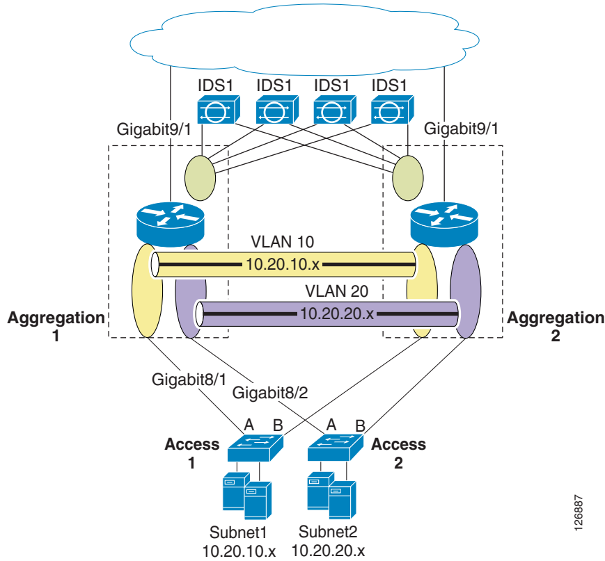
Figure 9-7 VLAN Topology
