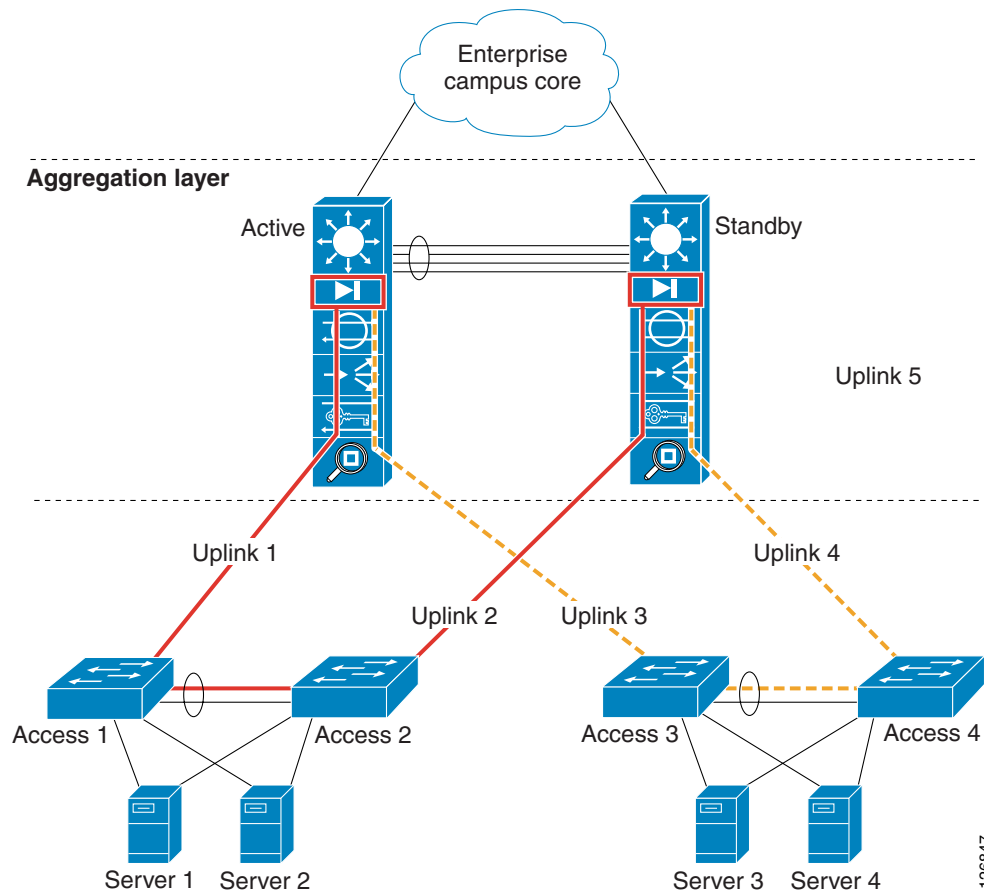
Figure 4-9 Incorrect FWSM Design
