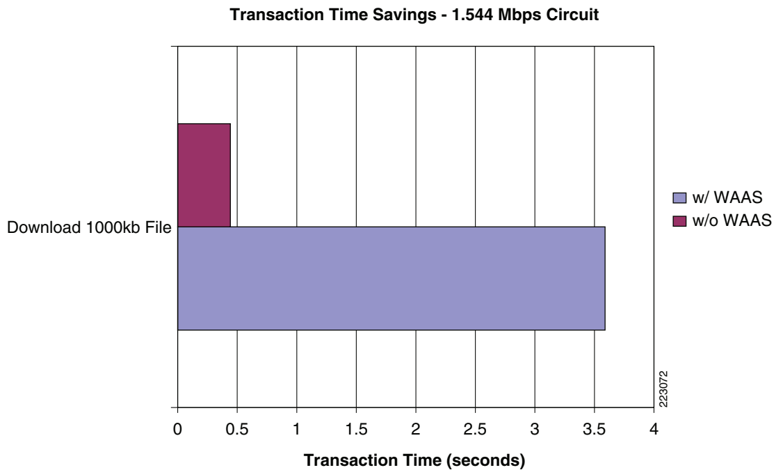
Figure 12 Transaction Time Savings 1.544 Mbps Circuit
