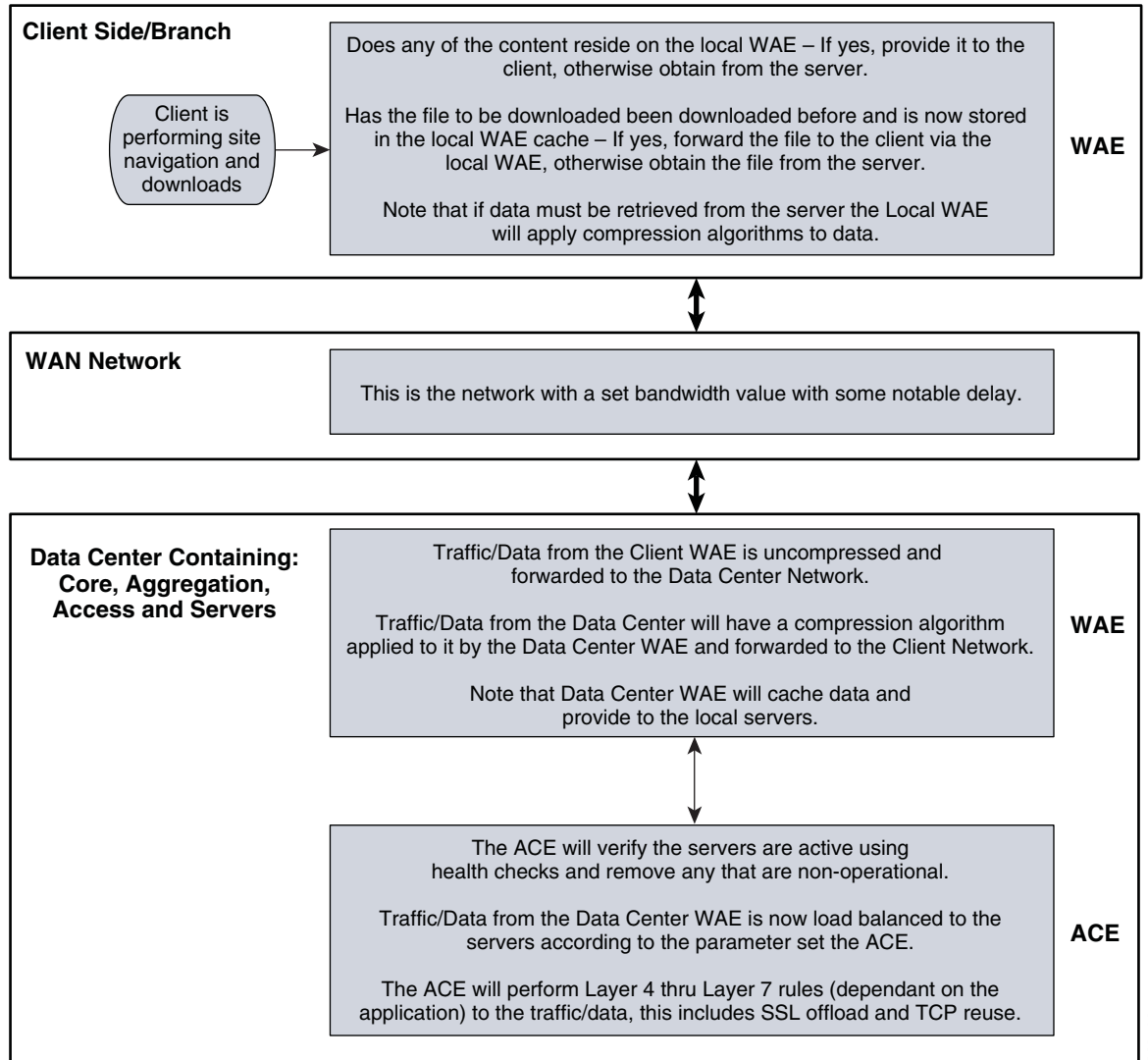
Figure 2 Process Flow
