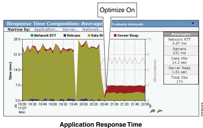
Figure 15 Benefit of Optimization Using the Cisco WAAS—Application Response Time
