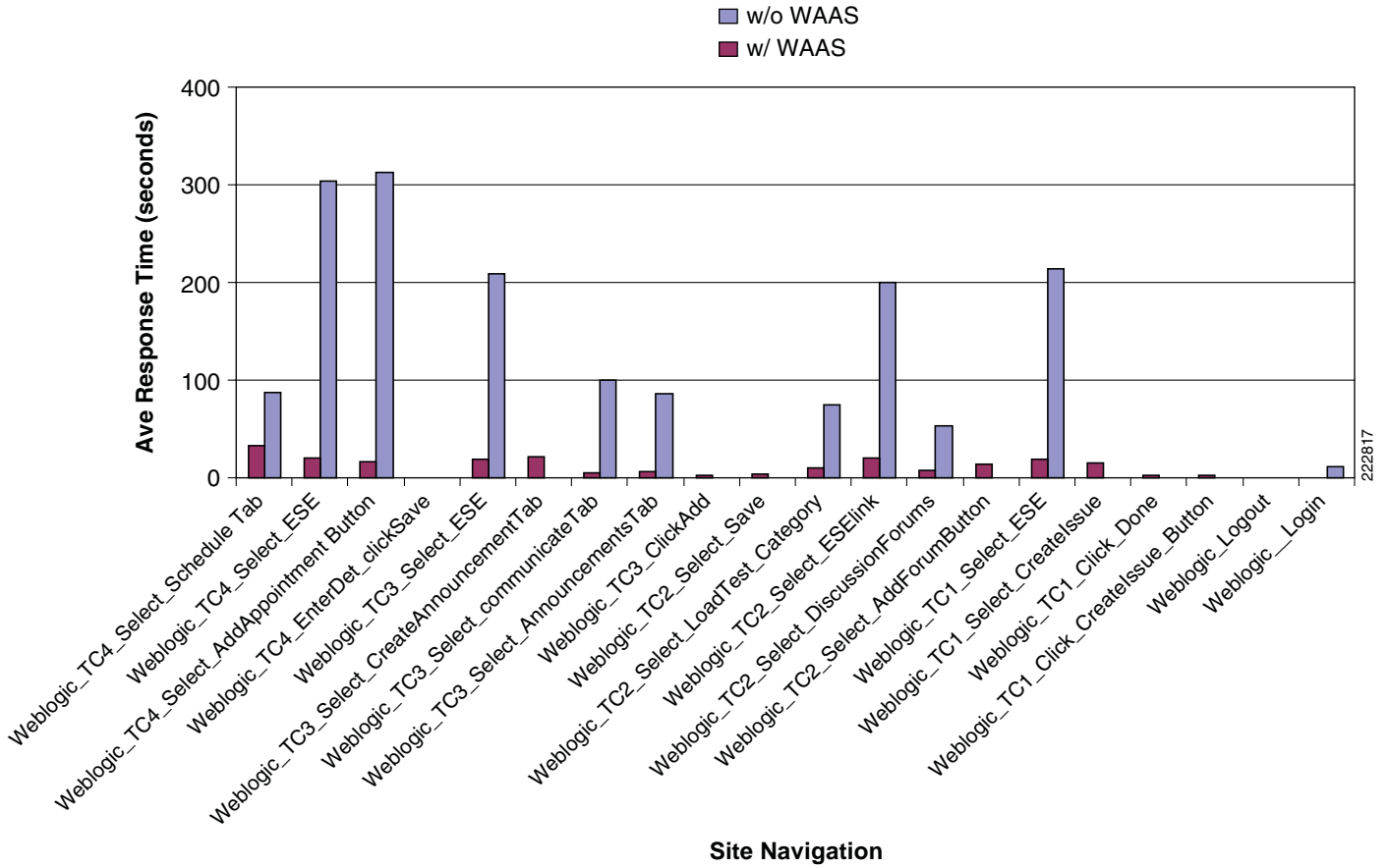
Figure 13 Response Time for 512 Kbps WAN Link
