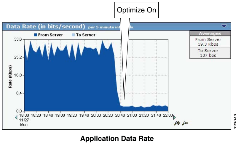
Figure 16 Benefit of Optimization Using the Cisco WAAS—Application Data Rate
