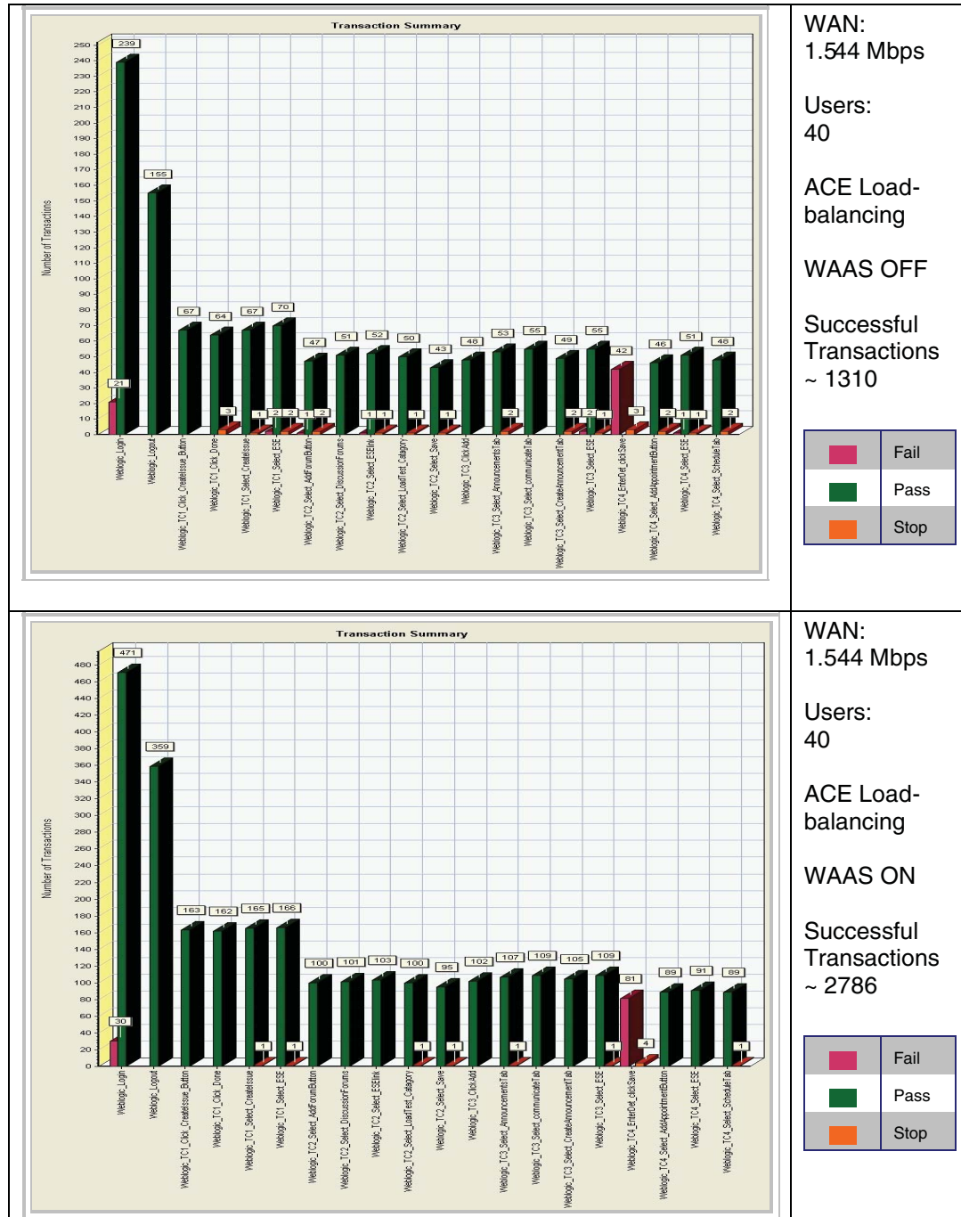
Figure 11 Number of Transactions for 1.544 Mbps WAN Link – With and Without Cisco WAAS
