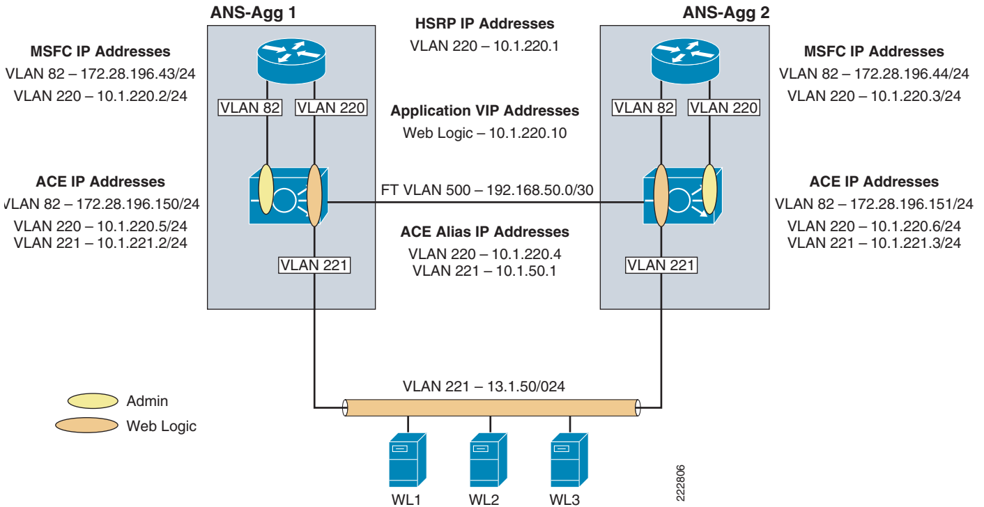
Figure 6 Network Topology
