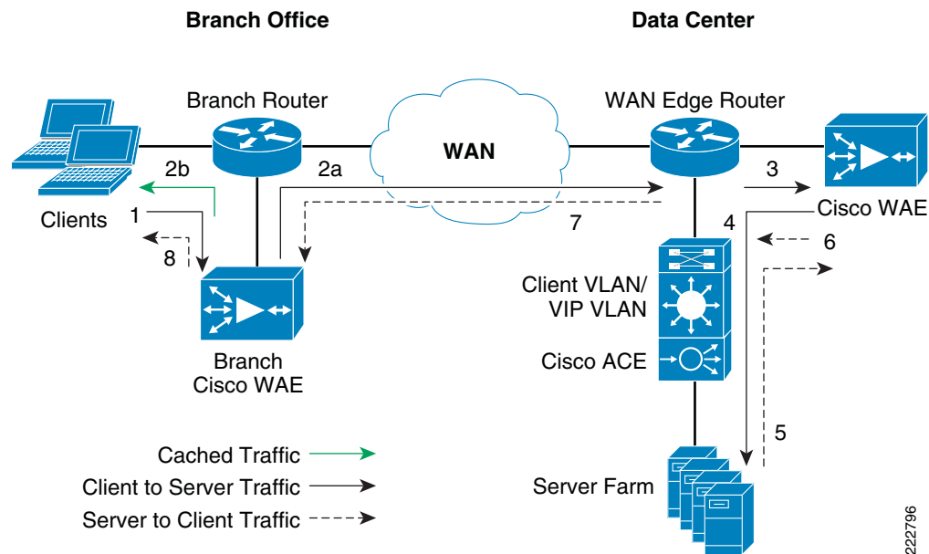
Figure 5 Packet Flow with Cisco WAAS and Cisco ACE
