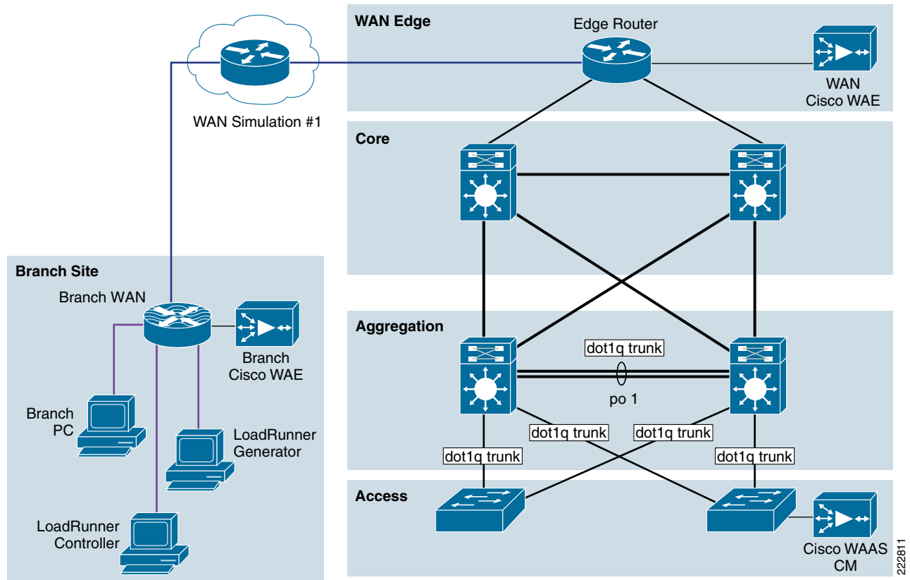
Figure 7 Network Topology
