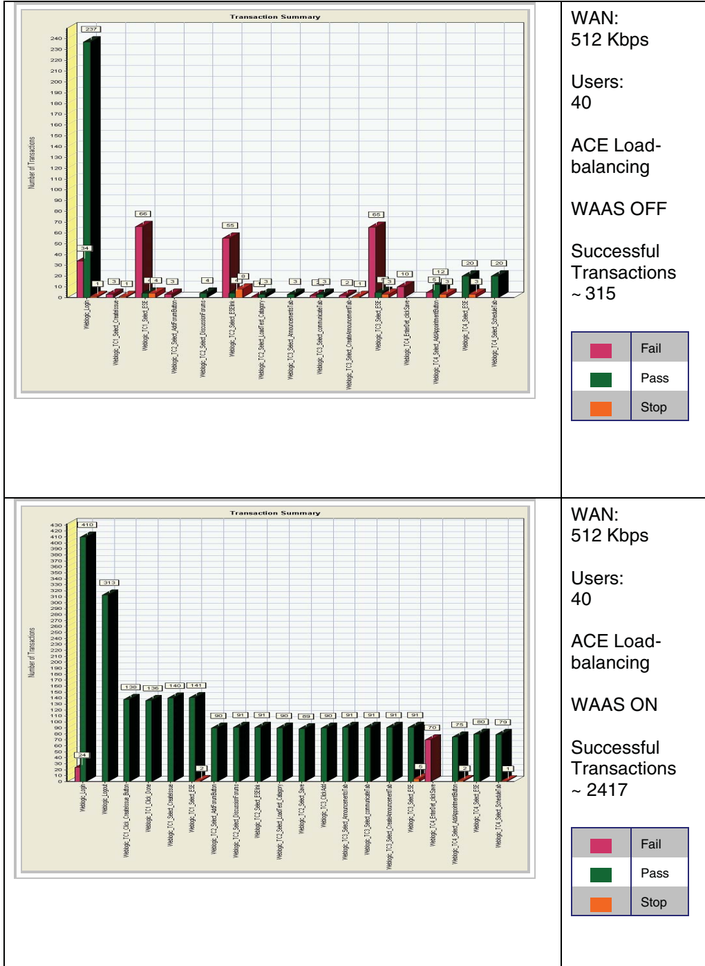
Figure 14 Number of Transactions for 512 Kbps WAN Link – With and Without Cisco WAAS
