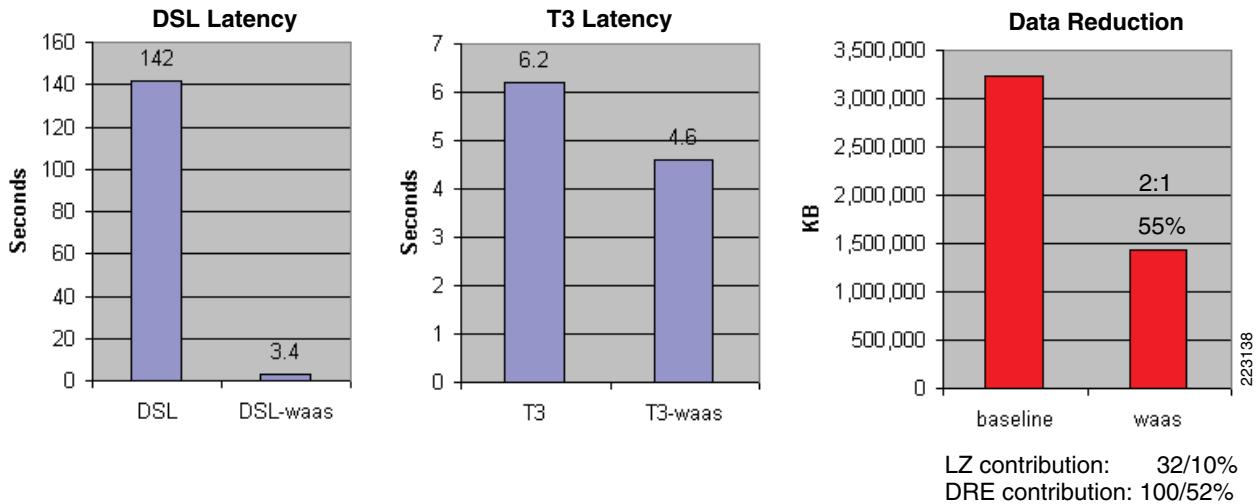
Figure 32 Summary Results for Login/Logout
