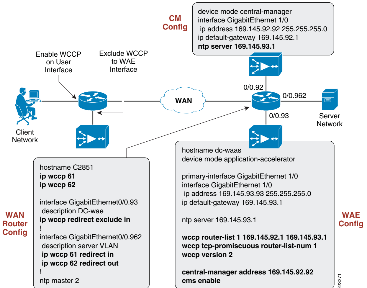
Figure 39 WAAS Configuration Summary
