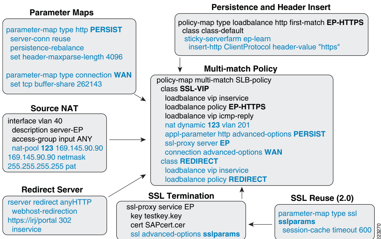
Figure 19 SAP Server Farm Deployment Optimization
