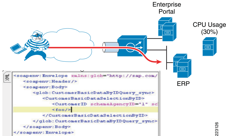
Figure 20 Denial-of-Service Attack with XML Schema Violation
