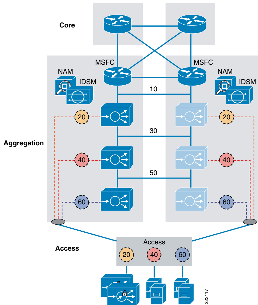
Figure 10 Data Center Architectural View
