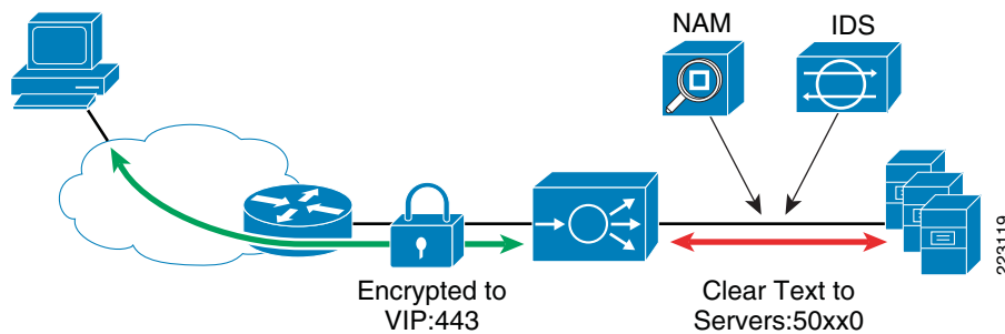
Figure 12 SSL Termination/Offload
