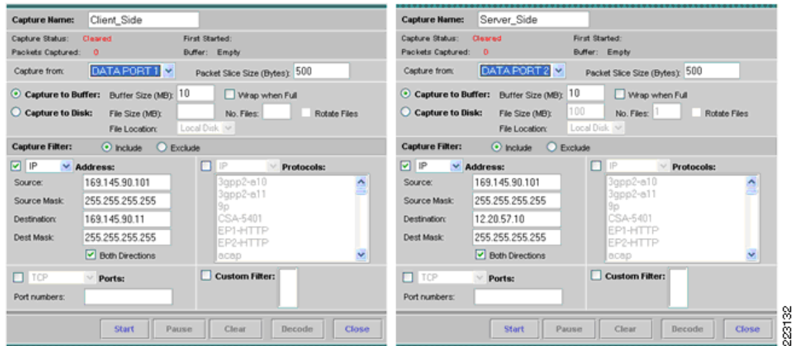
Figure 26 Cisco NAM Capture Setup
