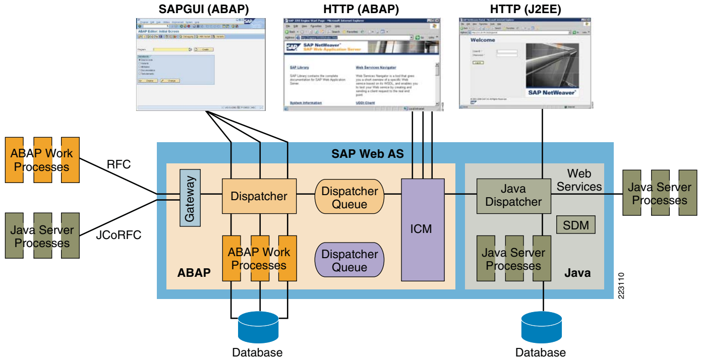
Figure 2 SAP Communications Patterns
