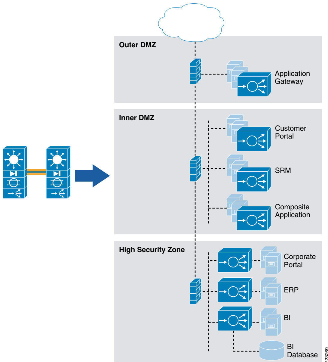
Figure 7 Infrastructure Consolidation with Virtualization
