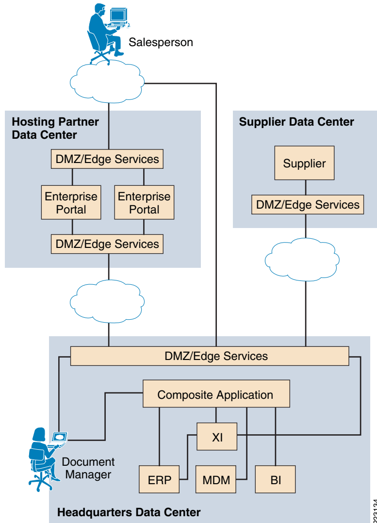
Figure 28 Enterprise SOA Communications across the WAN
