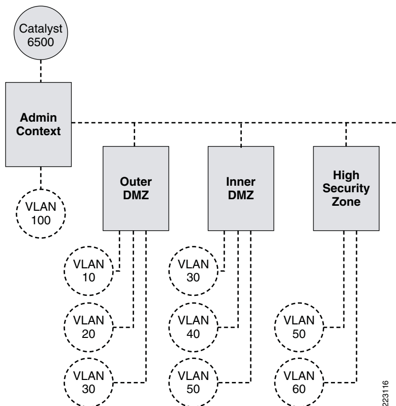
Figure 9 Cisco ACE Module Layout for SAP Server Farm
