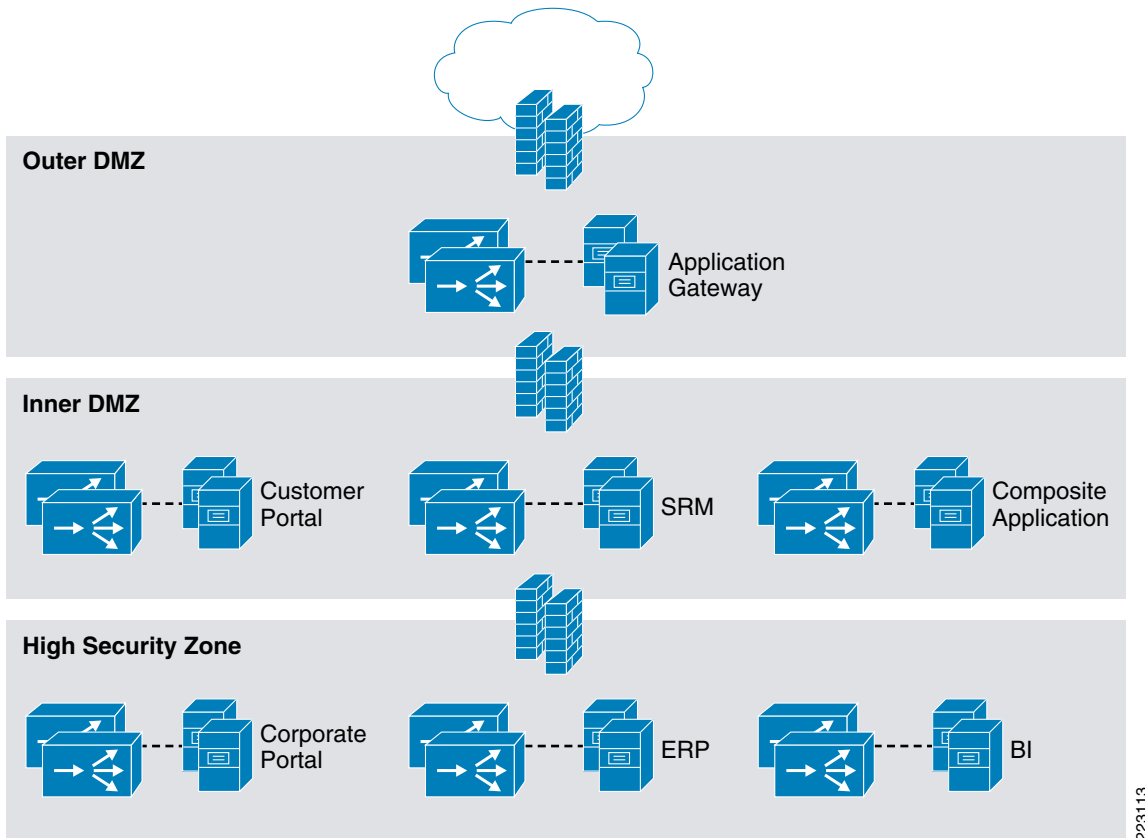
Figure 6 Deployment with Dedicated Firewalls and Load-Balancers
