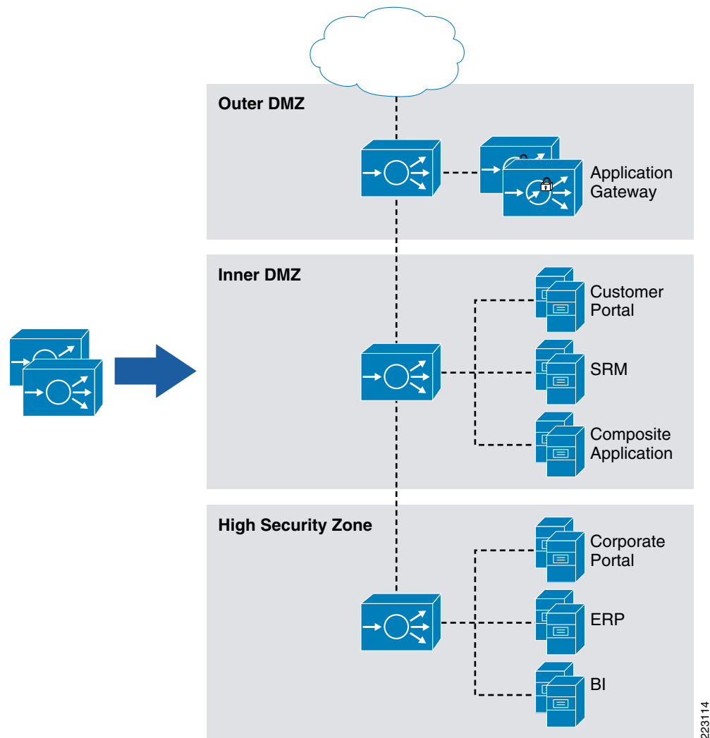
Figure 8 Deployment with Integrated Security, Load-balancing and SSL
