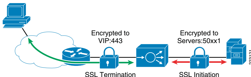
Figure 15 SSL Offload with Backend Encryption
