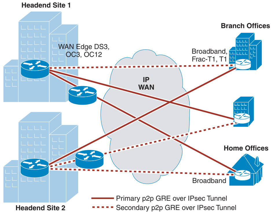
Figure 2-1 p2p GRE over IPsec—Single Tier Headend Architecture
