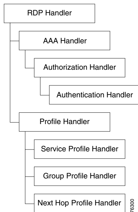
Figure 7-1 RDP Handlers
